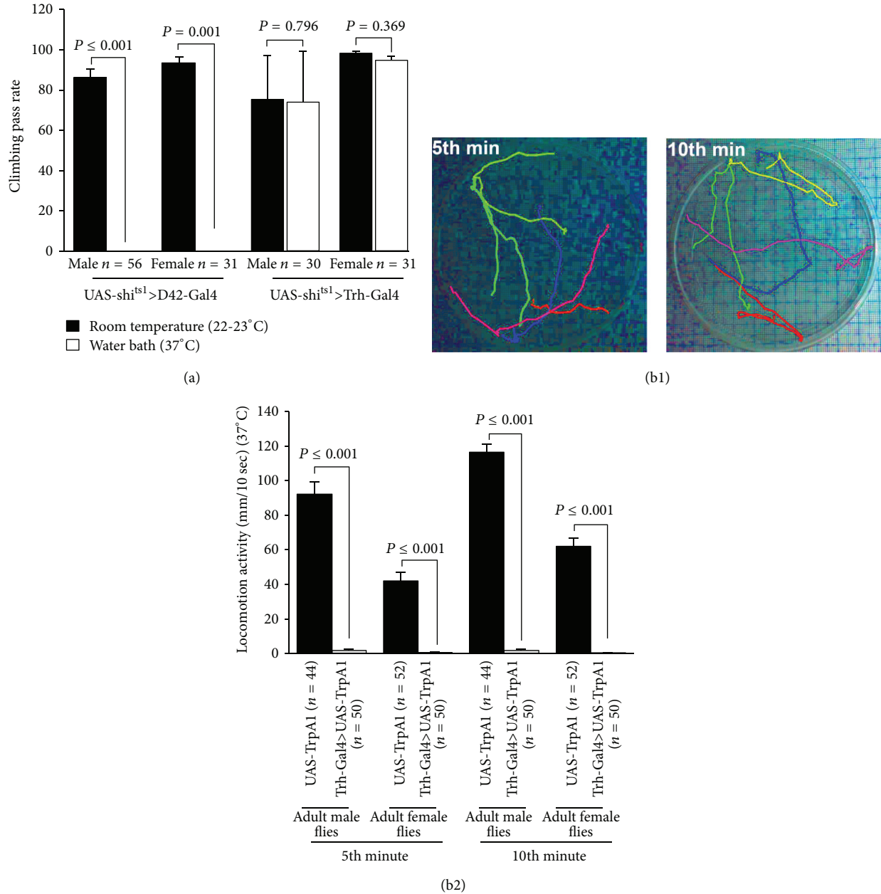
FIGURE 10: Manipulation of activity in 5-HTergic neurons within adult flies. (a) Acute inhibition of neuromuscular synapse neurotransmission by expressing shi tsl in motor neurons (UAS- shi tsl > D42-Gal4) significantly reduced climbing ability in adult female and male flies at restrictive temperature (37°C). This assay served as a proof of concept in the genetic crosses. However, acute blockage of serotonergic synaptic transmission (UAS- shi tsl > Trh-Gal4 (III)) did not influence climbing ability in adult flies. Student's t -test was used to compare the climbing ability of the flies at room temperature (22-23°C) with the same flies after incubation in the water bath (37°C). (b1) Locomotion activity was recorded for 10 minutes in UAS-TrpA1 (control) and Trh-Gal4 (III) > UAS-TrpA1, which expressed TrpA1 in 5-HTergic neurons, flies at 37°C. The activity was analyzed for 10 seconds at the 5th minute and 10 seconds at the 10th minute. These two pictures show the locomotion activity of adult male flies (controls), 10 sec of 5th and 10 sec of 10th minute, respectively. (b2) Acute activation of 5-HTergic neurons in freely moving adults significantly reduced the locomotion activity in adult male and female flies. Mann-Whitney rank sum test was used for comparison between the groups. Data represented as mean \pm SEM.
