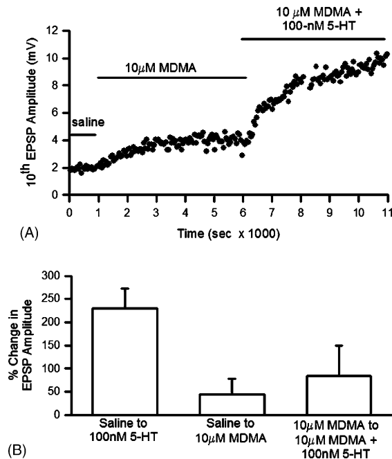
Fig. 2. Effect of MDMA on EPSP amplitude recorded from the opener muscle of crayfish. MDMA (10 \mu M) at the crayfish NMJ caused a gradual increase in the amplitude of the intracellular obtained EPSPs. (A) A 100 nM exposure of 5-HT to the crayfish NMJ enhances the 10th EPSP amplitude within a 40 Hz train by approximately 200%. (B) P < 0.05 , non-parametric rank sum Wilcoxon test). MDMA exposure at 10 \mu M produces a 45% increase of the 10th EPSP amplitude (A & B P < 0.05 , n = 5 preparations, non-parametric rank sum Wilcoxon test). Exposure of the NMJ preparation to MDMA (10 \mu M) combined with 5-HT (100 nM) after the preparation had already been exposed to MDMA (10 \mu M) produces an 84% enhancement of the EPSP amplitude (B).
