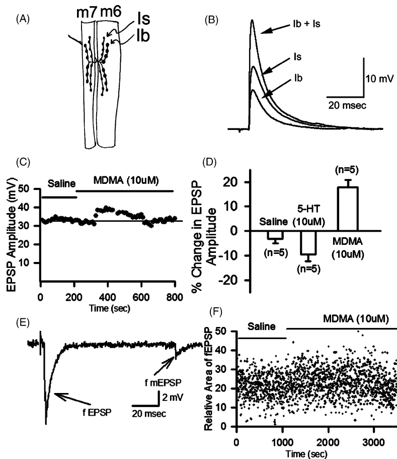
Fig. 4. The Drosophila larval neuromuscular preparation. Muscle 6 of the third instar Drosophila larvae has two motor nerve terminals that innervate it (A). The Is axon gives rise to large EPSPs in the muscle, whereas the Ib axon produces smaller EPSPs (B). MDMA enhances the combined amplitude of the Ib & Is EPSP transiently (C). 10\ \mu\text{M} exposure of 5-HT resulted in a slight but non-significant decrease on the amplitude of the composite Ib and Is EPSP when compared to saline controls over the same time period (D). The amplitudes of the EPSPs drop slightly over time in non-voltage clamped Drosophila preparations. MDMA ( 10\ \mu\text{M} ) produced a slight enhancement of the EPSP amplitude in each preparation examined ( P < 0.05 , n = 5 preparations, non-parametric rank sum Wilcoxon test). With focal macropatch recordings over distal Is varicosities the multiquantal evoked release fEPSP and spontaneous quantal events (fmEPSP) are able to be measured (E). An increase in evoked release occurs due to exposure of MDMA ( 10\ \mu\text{M} ) (F). Although the changes are small there is a consistent increase in the area of the fEPSPs after exposure to MDMA without any measurable differences in characteristics of spontaneous events.
