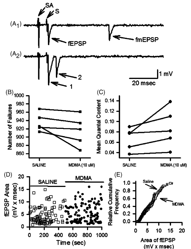
Fig. 3. Quantal recordings from defined regions of the excitatory motor nerve terminal on the opener muscle. Quantal releases were monitored by directly counting the number of quantal events in the field excitatory postsynaptic potentials (fEPSPs) obtained in focal macropatch recordings from defined regions of the motor nerve terminals. The stimulus artifact (SA), the nerve terminal spike (S), and a single evoked response are readily measured (A 1 ). Two evoked events are shown in the trace (A 2 ). The number of failures in evoking a response decreased upon exposure to MDMA (B) P < 0.05 , n = 5 preparations, non-parametric rank sum Wilcoxon test. Mean quantal content for 1000 stimulus trials prior to and during exposure to MDMA (10 \mu M) increased upon exposure to MDMA (C) P < 0.05 , non-parametric rank sum Wilcoxon test. Measures of the area under the trace for evoked single fEPSPs before and during exposure showed no differences in the area distributions (D). Upon normalization for the number of increased events during exposure to MDMA, the relative cumulative frequency plot in the areas of the single fEPSPs showed no substantial shifts in the distributions, implying that MDMA has no effect on postsynaptic receptivity of released glutamate (E).
